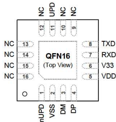
Figure 3–2. MA112 QFN16 (4x4) Top View
