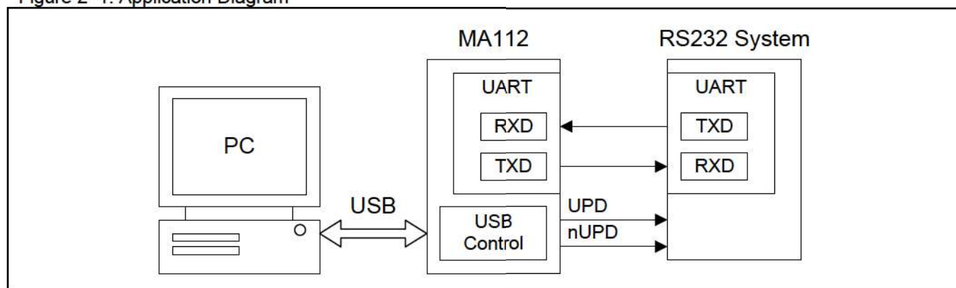
Figure 2–1. Application Diagram
